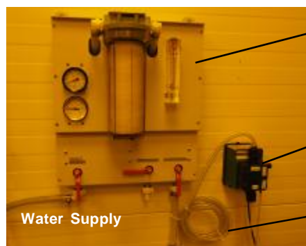
Dosing Pump
